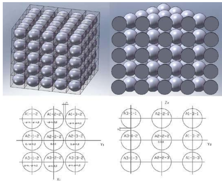
Fig. 5: The supposed distribution structure of pores with a single diameter
